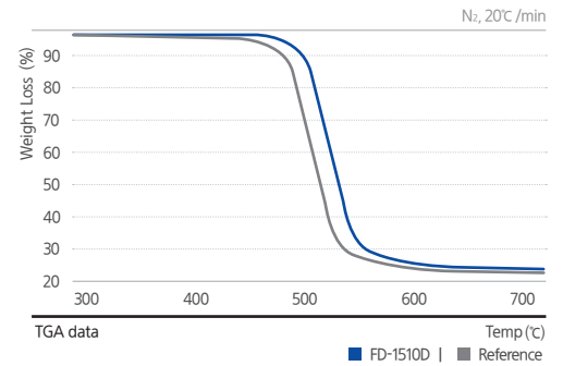
Thermal Stability
